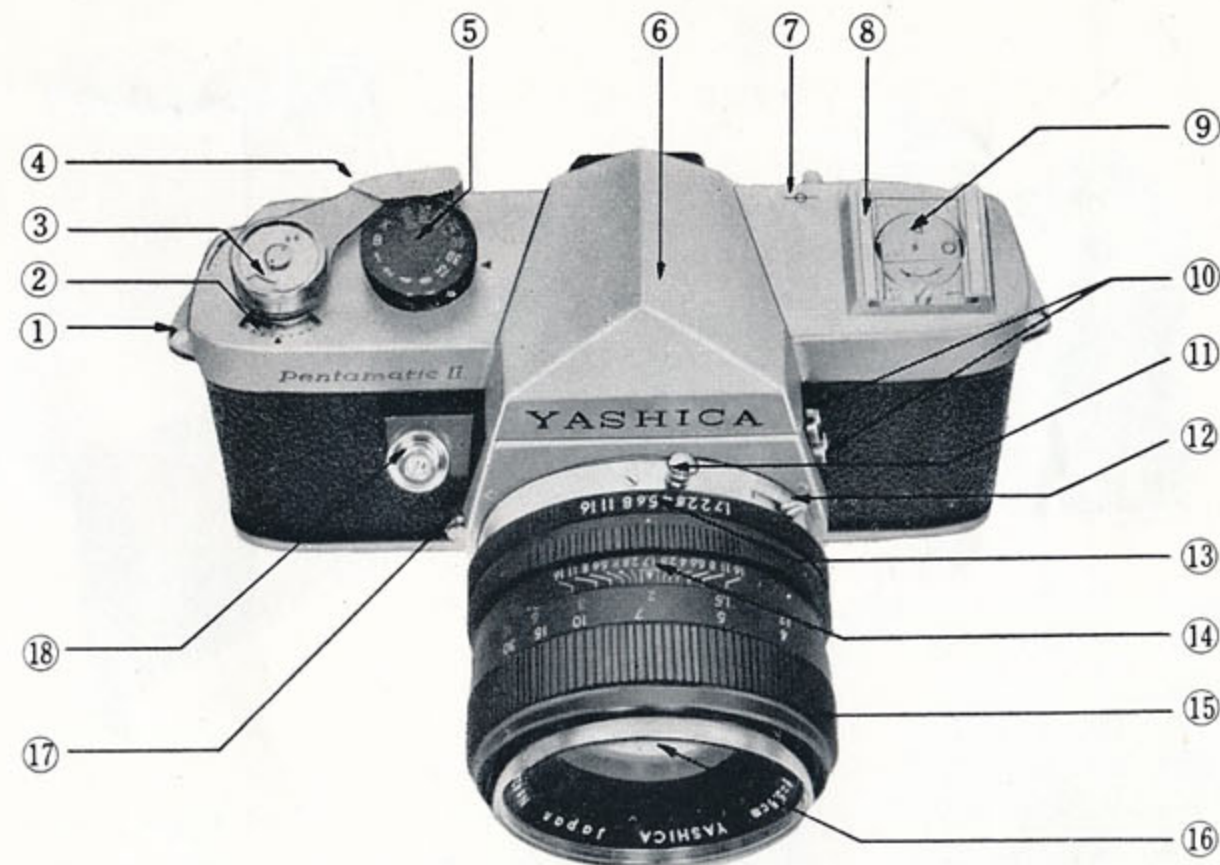
YASHICA Pentamatic 35 mm Single lens Reflex
